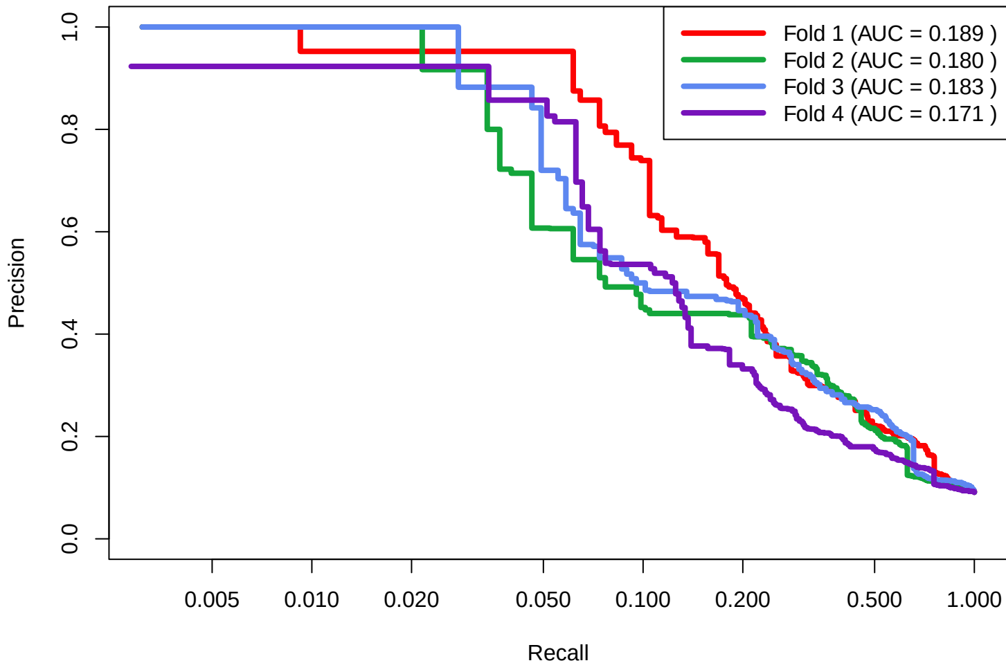
SPELL All Datasets: 430x20x10x1 Fold Set 3
